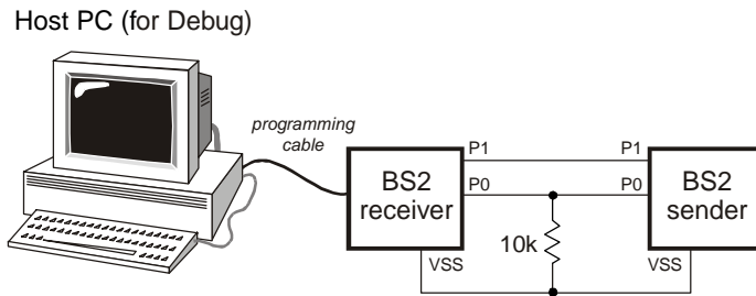
Figure 5.33: Flow-Control Example Circuit.
